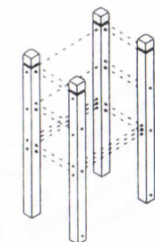
(A) Upper Post (Shorter) x 4
