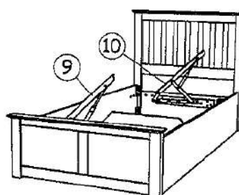
5.2 Hydraulic Base Support installation for OPTION 2
